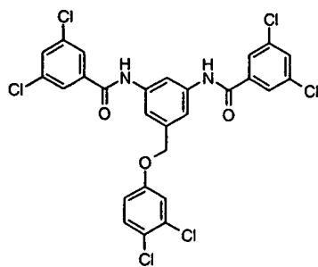
Compound # 6
